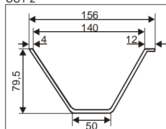
CUT 2
