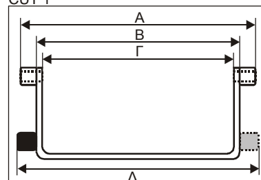
CUT 1
